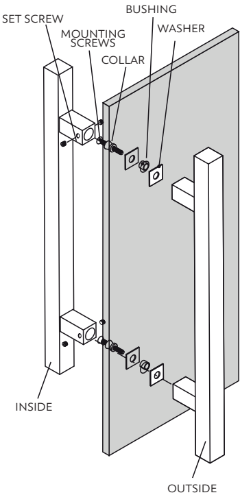
Back-to-Back Handle
